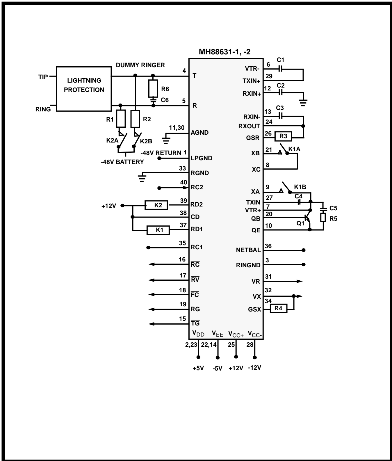
Figure 3 - Application Circuit
