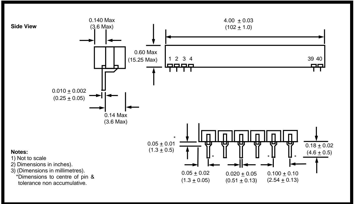
Figure 4 - Mechanical Data
